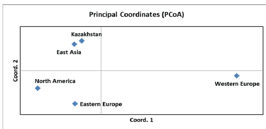
Fig. 5. Principal coordinate analysis of 288 soybean accessions divided into 5 groups based on 9 SSR markers associated with the resistance to fungal diseases
